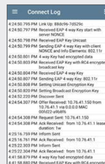
Connect Log shows roam/association process
